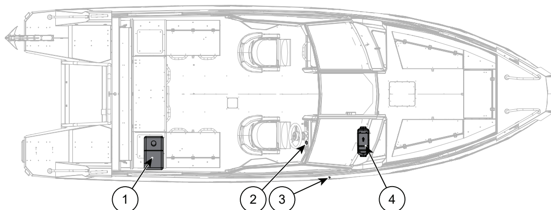
Figur 6.2 Buster Magnum/SuperMagnum varmeapparat
