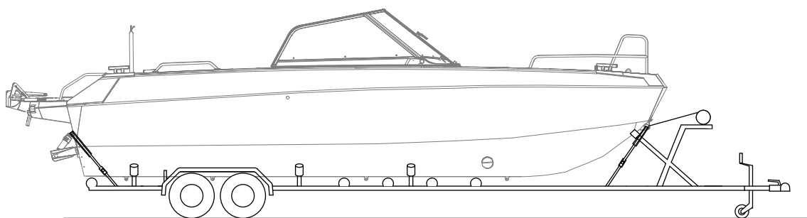
Figur 12.1 Buster Magnum/SuperMagnum tilhengertransport
